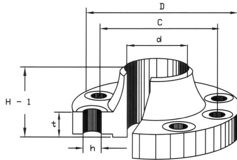
Weld-Neck
